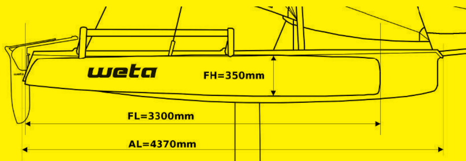
Diagram 2: Dimensions of Hulls – Side View
